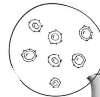
The smallest possible bubbles stabilised by proteins
